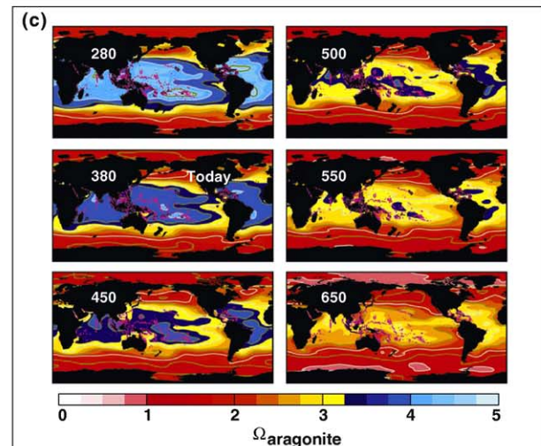
Figure 1. Chemistry of ocean acidification and global changes in aragonite saturation. (a) Schematic view of the anthropogenic perturbation of the carbon cycle in which part of the CO 2 emitted from the combustion of fossil fuels and deforestation is absorbed by the oceans. (1) Chemical equilibrium reactions in which CO 2 intervenes as it dissolves in seawater, where K_1 and K_2 are the dissociation constants for carbonic acid and bicarbonate ion, respectively. (2) Definition of the saturation state ( \Omega ), where K_{\text{sp}} is the solubility constant of each mineral phase. (3) Calcium carbonate precipitation reaction that illustrates the release of CO 2 as precipitation occurs. (b) Near past (1800) and near future (2100) evolution of surface pH (orange, on total scale) and atmospheric CO 2 (magenta) from [10] based on prescribed fossil-fuel and land-use CO 2 emissions from historical data for the period 1820 to 2000 and considering the A2 IPCC SRES emissions scenario afterwards. Evolution of bicarbonate (green) and carbonate ion (blue) concentrations, computed from dissolved inorganic carbon and pH data from [10]. These calculations were done using the CO2SYS.XLS program (Pelletier et al. , available at www.ecy.wa.gov/programs/eap/models.html ). The grey cloud of points shows all 1 \times 1 degree mixed surface layer (upper 50 m) pH values in the oceans, computed from total carbon and alkalinity data (see Box 4 for more details). (c) Reconstructions for the past and present, and predictions for the future changes in the aragonite saturation state ( \Omega , equation (2) in Figure 1a) at different levels of atmospheric CO 2 concentrations (white numbers in ppmv; reprinted with permission from [5]). Note the dramatic reduction in blue areas, which are representative of the approximate minimum \Omega_{\text{aragonite}} values needed for carbonate coral reef communities to develop properly [83].
